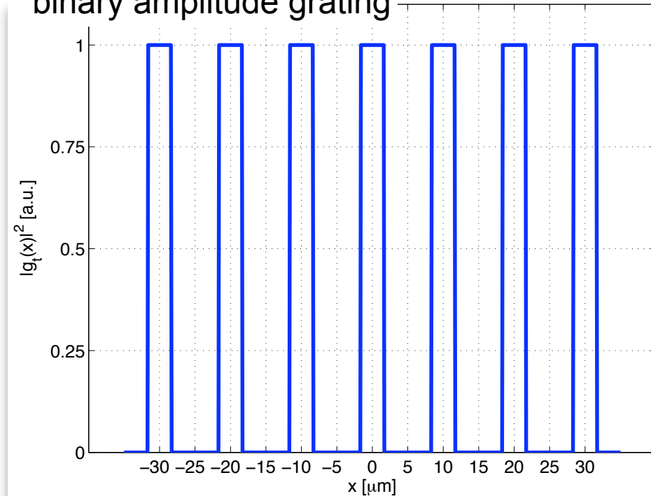
binary amplitude grating
