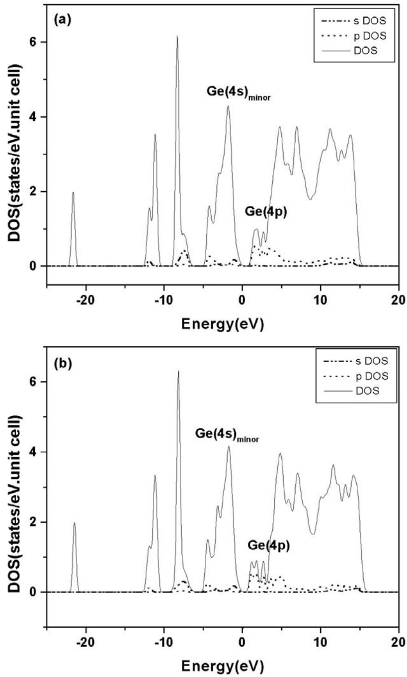
Figure 4. (a) The partial densities of states (DOS) of the Ge-atom contributions in \text{CsGeI}_3 ( R3m ). (b) The partial densities of states (DOS) of the Ge-atom contributions in \text{CsGeI}_3 ( Pmmm ).
