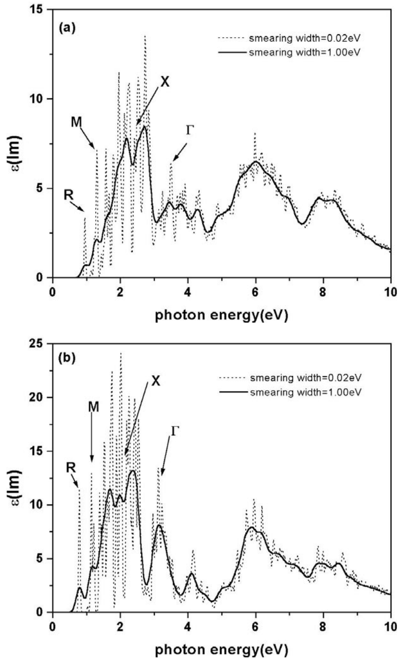
Figure 6. (a) The dispersion of the imaginary part of the dielectric constant in \text{CsGeI}_3 ( R3m ). (b) The dispersion of the imaginary part of the dielectric constant in \text{CsGeI}_3 ( Pmmm ).
