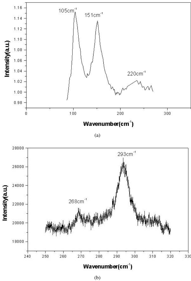
Figure 10. (a) A Raman spectrum of \text{CsGeI}_3 ( R3m ) single crystal. \lambda_{exc} = 488.7 nm. There are two major peaks, at 105\text{ cm}^{-1} and 151\text{ cm}^{-1} , detected with a spectral range from 100\text{ cm}^{-1} to 200\text{ cm}^{-1} . (b) A Raman spectrum of \text{CsGeI}_3 ( R3m ) single crystal. \lambda_{exc} = 514.5 nm. There are two major peaks, at 268\text{ cm}^{-1} and 293\text{ cm}^{-1} , detected with a spectral range from 250\text{ cm}^{-1} to 320\text{ cm}^{-1} .
